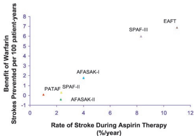
Figure 2. Advantage of anticoagulation over aspirin for patients with atrial fibrillation in 6 randomized trials: PATAF, 249 SPAF II, 247 AFASAK II, 254 AFASAK I, 241 SPAF III, 124 and EAFT. 246
